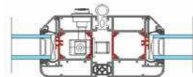
Interlock Detail
